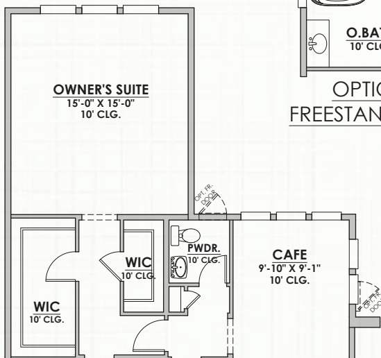
OPTIONAL POWDER BATH NOTE: SPACE REMOVED FROM WIC & CAFE
