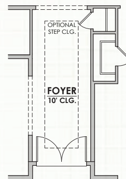
OPTIONAL DOUBLE ENTRY DOORS
