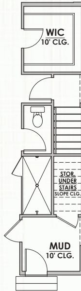
FIRST FLOOR STAIR LOCATION W/OPTIONAL BONUS ROOM
